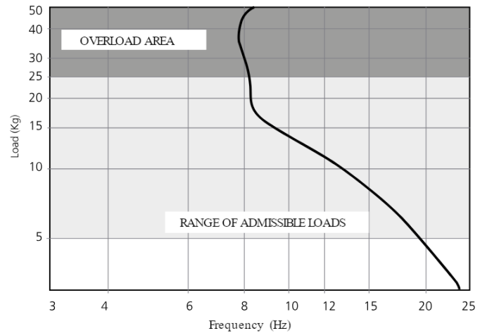
NATURAL FREQUENCY GRAPH EP Akustik+Sylomer®
