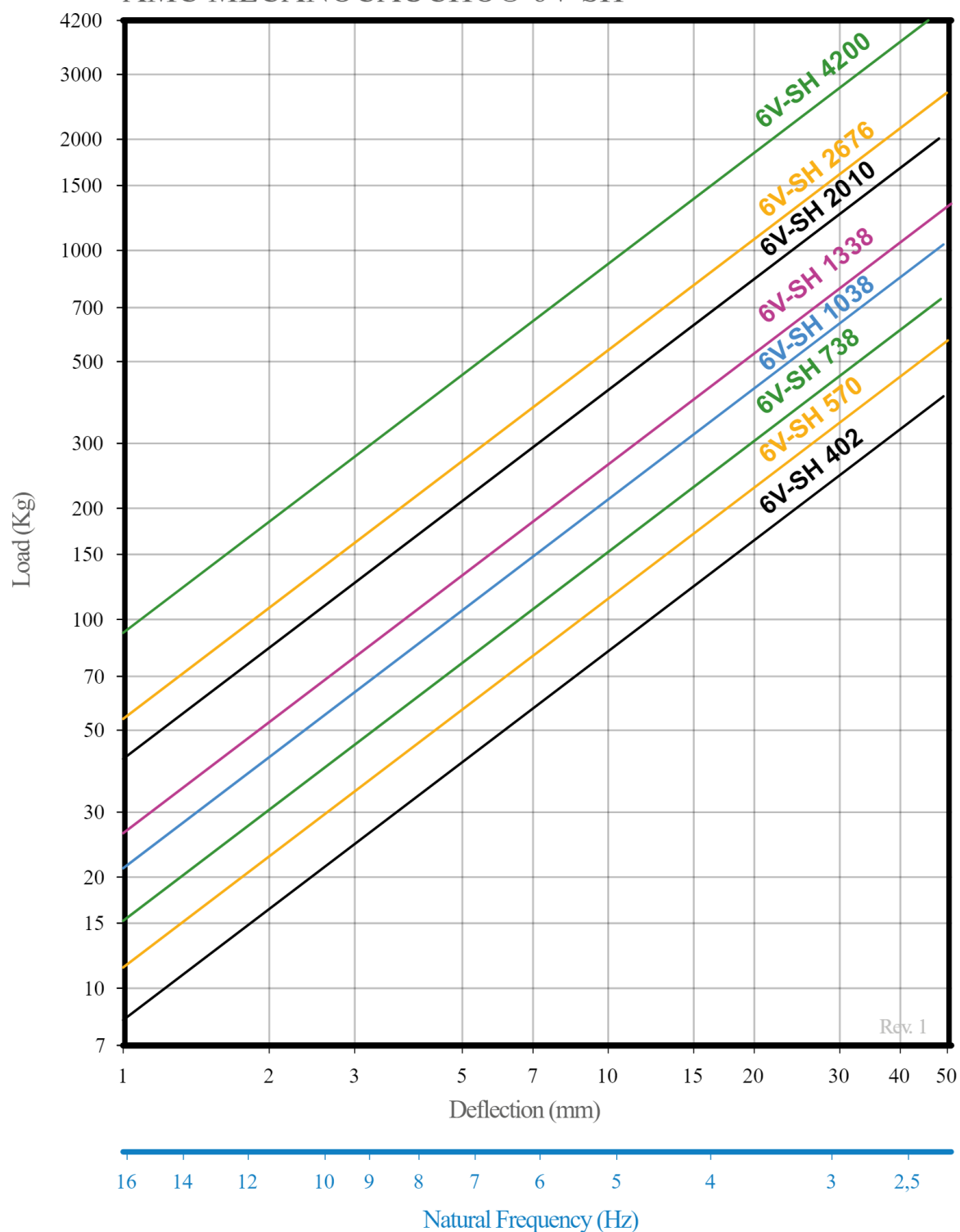
LOAD DEFLECTION GRAPH AMC MECANOCAUCHO® 6V-SH
