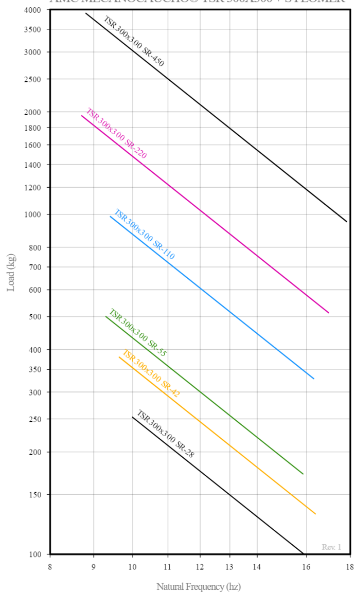
NATURAL FREQUENCY AMC MECANOCAUCHO® TSR 300X300 + SYLOMER
