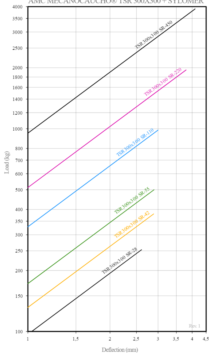
LOAD DEFLECTION AMC MECANOCAUCHO® TSR 300X300 + SYLOMER
