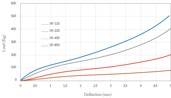
TRACTION LOAD DEFLECTION
