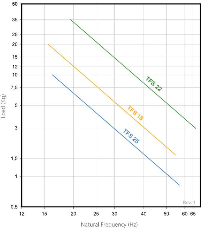
NATURAL FREQUENCY GRAPHS AMC MECANOCAUCHO® TFS ANTI VIBRATION MOUNTS
