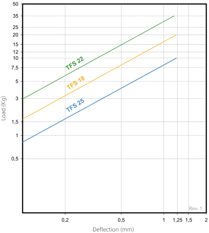
LOAD DEFLECTION GRAPHS AMC MECANOCAUCHO® TFS ANTI VIBRATION MOUNTS
