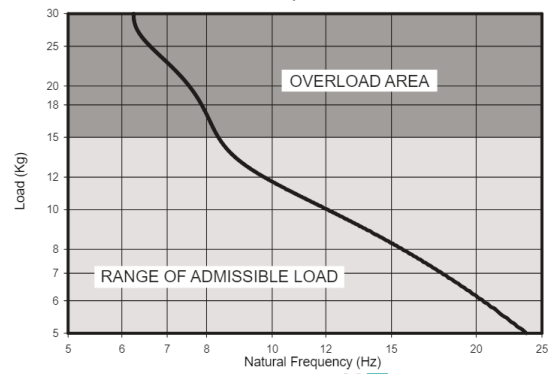
NATURAL FREQUENCY GRAPHS
