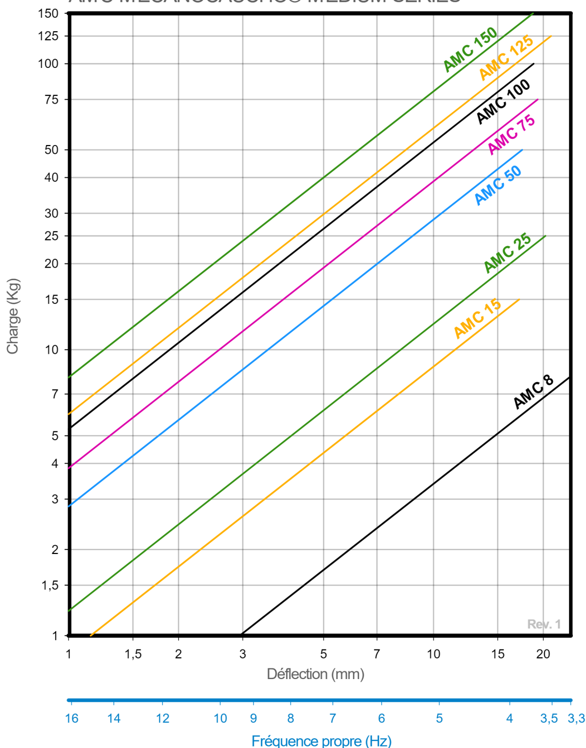
COURBE DE CHARGE FLÈCHE AMC MECANOCAUCHO® MEDIUM SERIES
