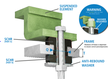
ASSEMBLY 2
