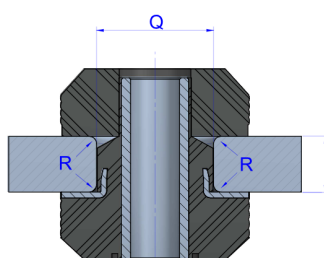
ASSEMBLY DETAIL
