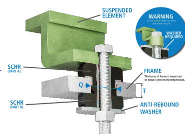
ASSEMBLY 2
