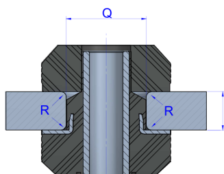
ASSEMBLY DETAIL
