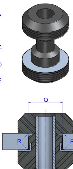
ASSEMBLY DETAIL
