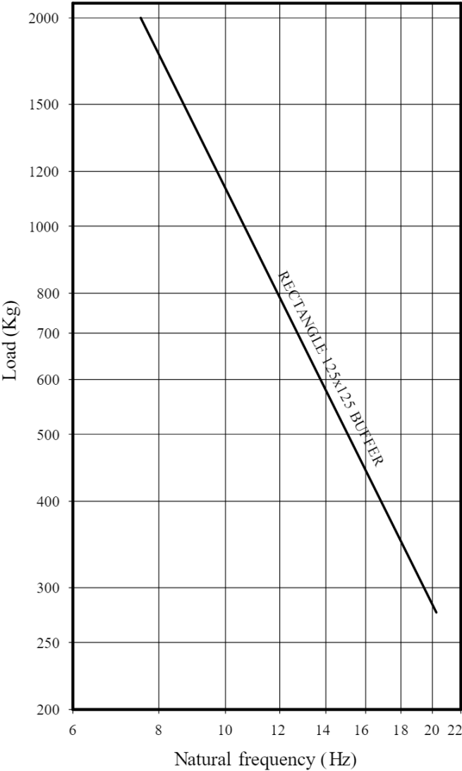
NATURAL FREQUENCY CURVES RECTANGLE 125x125 BUFFER
