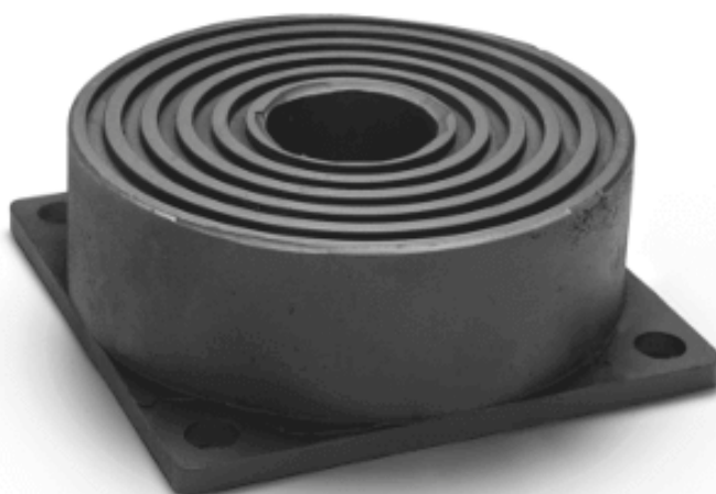
AMC-MECANOCAUCHO® Type P Anti-Slip Anti-Vibration Mount
