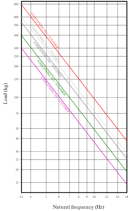
NATURAL FREQUENCY CURVES FZHM SPRING + SYLOMER®
