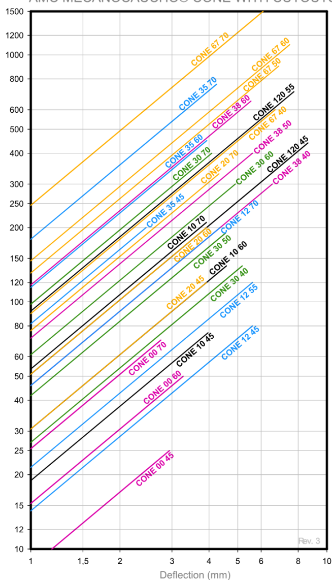
LOAD DEFLECTION GRAPH AMC MECANOCAUCHO® CONE WITH CUTOUTS
