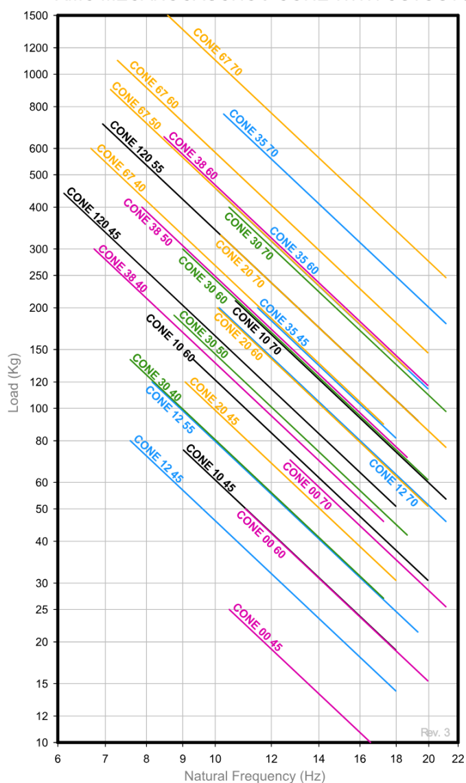
NATURAL FREQUENCY AMC MECANOCAUCHO® CONE WITH CUTOUTS
