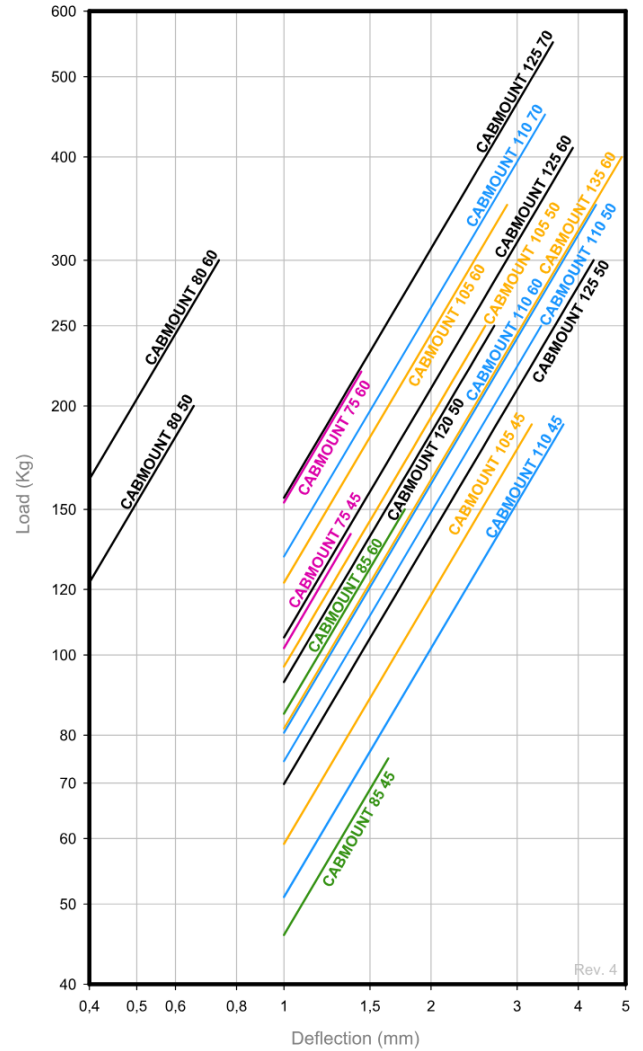
LOAD DEFLECTION GRAPHS AMC MECANOCAUCHO® CAB MOUNT
