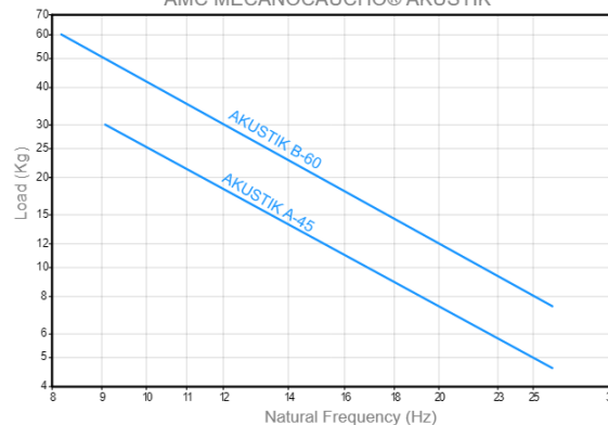
NATURAL FREQUENCY AMC MECANOCAUCHO® AKUSTIK
